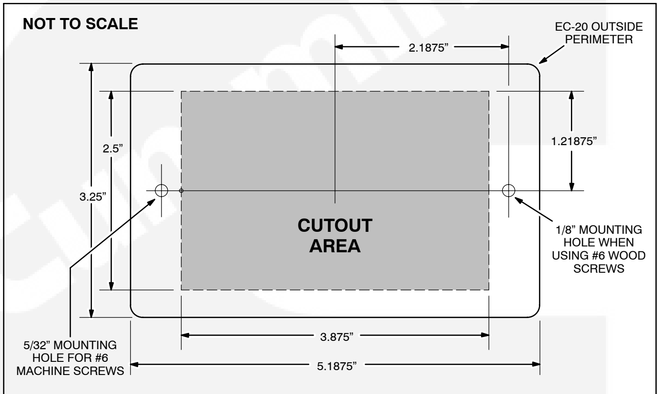
Mounting Footprint
